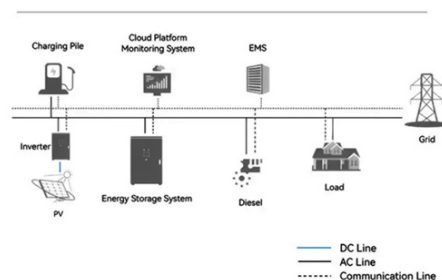
System Topology
